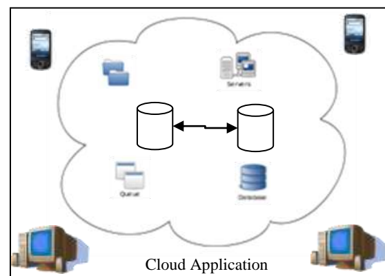
Figure 1: Cloud Computing
