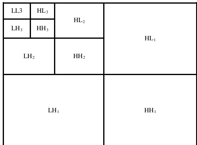
Fig.2.1: DWT on 2-dimensional data
