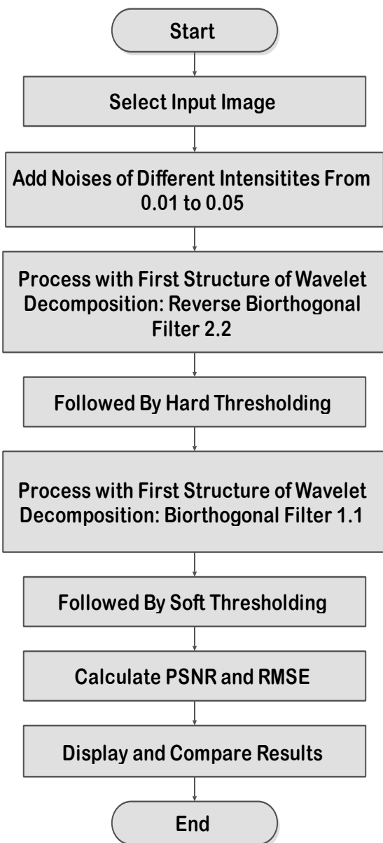
Fig. 3.2: Flow Chart of Proposed Methodology
