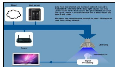
Figure 1: Block diagram of Lifi technology.
