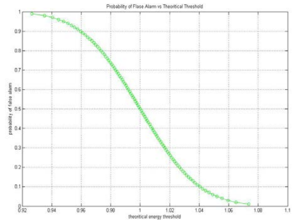
Fig.5.4 Probability of False Alarm w.r.t. theoretical threshold
