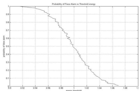
Fig.5.3 Practical Probability of False Alarm
