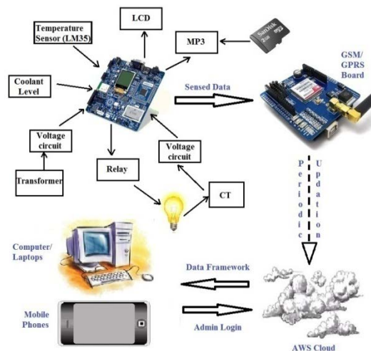
Fig. 2.1 System Architecture
