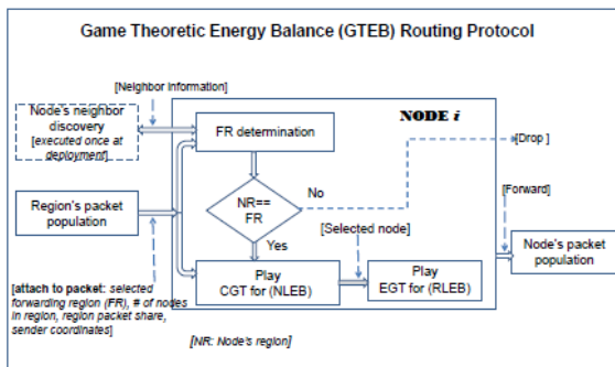
Fig.3 Functional Diagram
