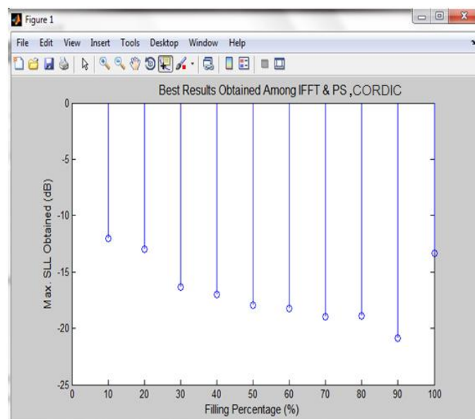
Figure 5. Graph Showing Best Results Obtained Among IFFT & PS, CORDIC
