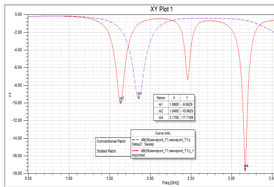
Figure 3.1 Return loss S_{11} vs. frequency plot of Conventional and slotted patch antenna.
