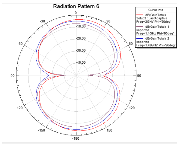
Figure 10 Gain pattern for DGS 3 at 1.1, 1.42 and 2 GHz.
