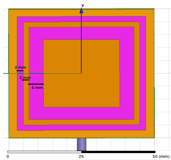
Figure 5. DGS2 Ground Plane
