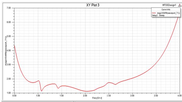
Figure 9: VSWR vs. frequency plot DGS3 antenna.
