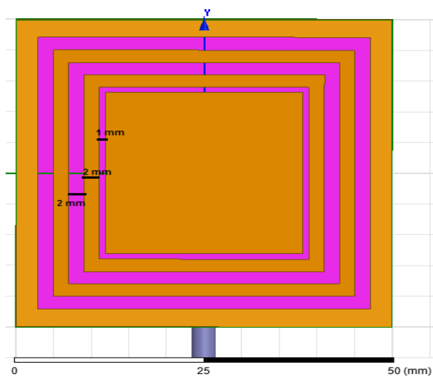
Figure 6 DGS3 Ground plane
