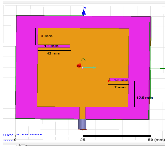
Figure 2: The configuration of slotted patch of the proposed for 1.85 and 3.2 GHz .
