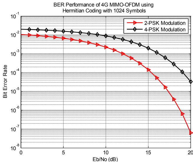
Fig. 4.3 BER Performance Curve for 4G MIMO System using Hermitian Encoding with 1024 number of Symbols
