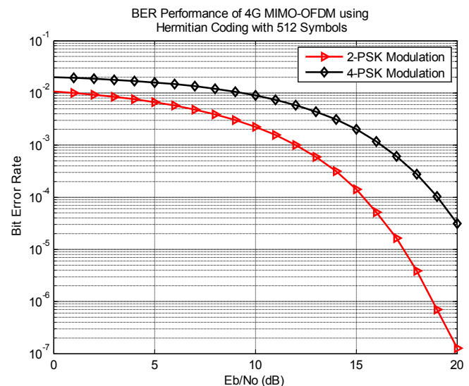
Fig. 4.2 BER Performance Curve for 4G MIMO System using Hermitian Encoding with 512 number of Symbols
