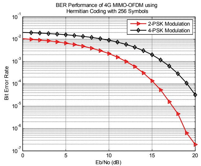
Fig. 4.1 BER Performance Curve for 4G MIMO System using Hermitian Encoding with 256 number of Symbols
