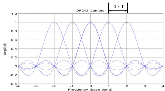
Fig. 2.1 Frequency spectrum of OFDM
