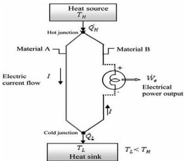
Figure 7- Circuitry of thermoelectric power
