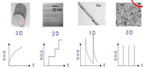
Figure 4- Dimensional view of material
