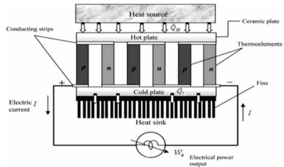
Figure 6- Thermoelectric effect
