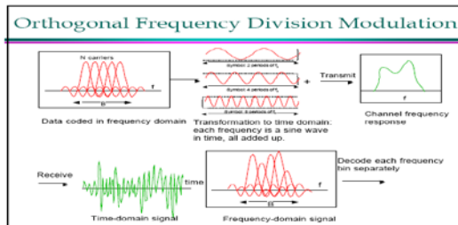
Figure 1 OFDM signal
