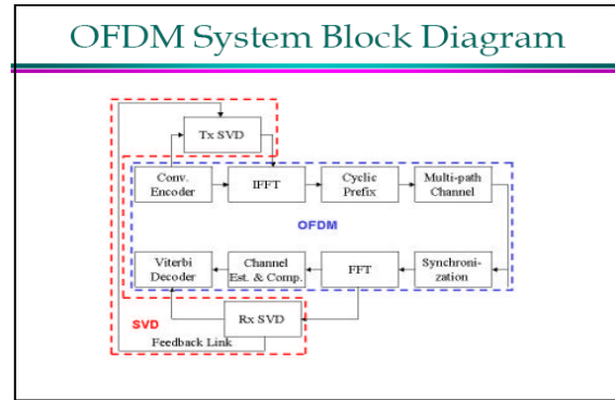
Figure 4. Block diagram of OFDM
