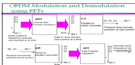
Figure 3. Modulation and Demodulation in OFDM
