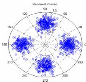
Figure 7. OFDM received signals Plots.
