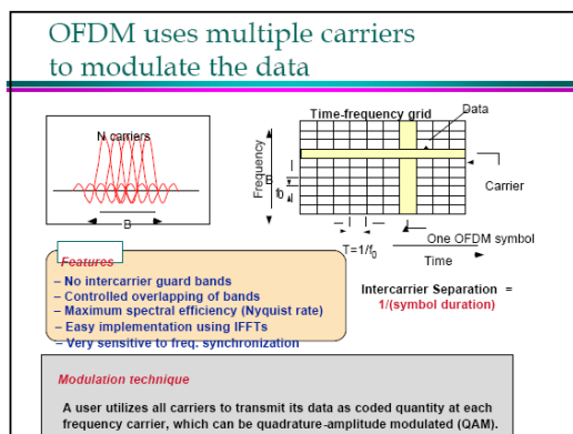
Figure 2 Basics of OFDM
