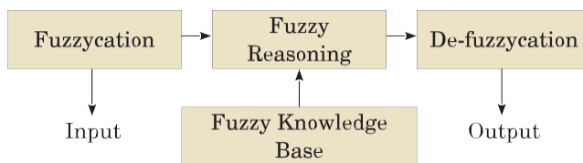
Fig. 3. Fuzzy Logic
