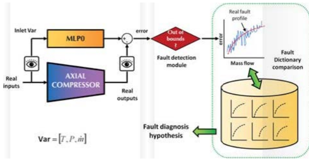
Fig. 1. Fault Detection Mechanism
