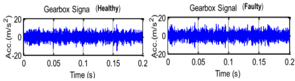
Figure 2.1-Waveform of the vibration signal for a gearbox with healthy and faulty gears
