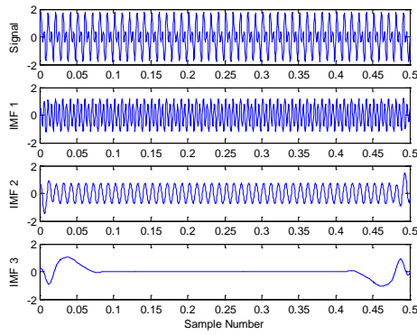
Fig 3.1. Empirical mode decomposition of the simulated signal x[n]
