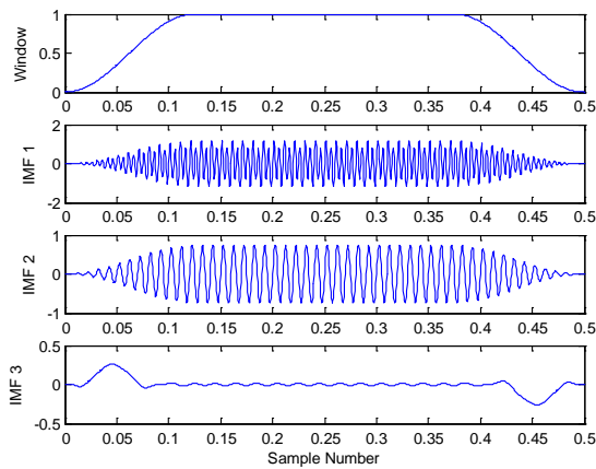
Fig 3.2. Windowing of IMFs of the signal x[n]
