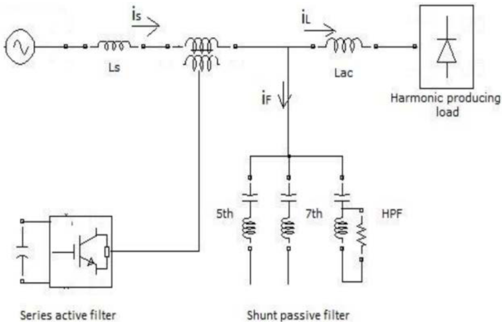
Figure 2.2 Combination of series active filter and shunt passive filter.
