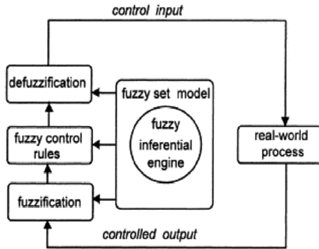
Fig.2.3 Fuzzy Logic Controller Architecture.
