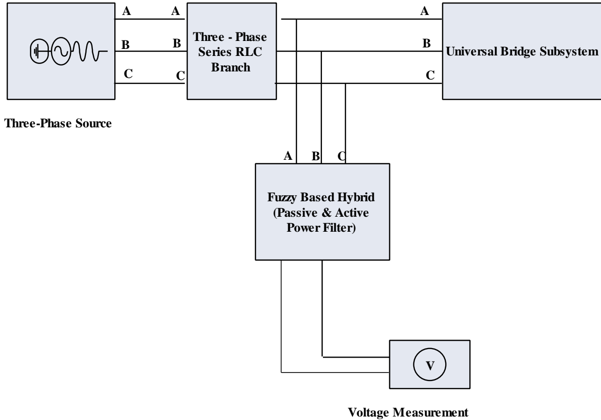
Figure 2.1 Typical Block Representation of Proposed work.
