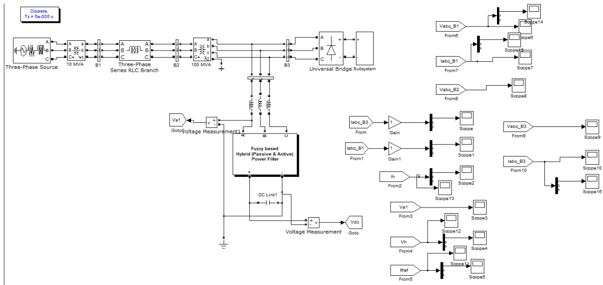
Figure 2.4 Proposed simplified model with Hybrid (active & passive power filter)
