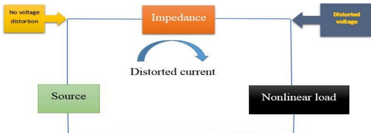
Figure 1.1 Flow of harmonic currents and generation of harmonic voltages.
