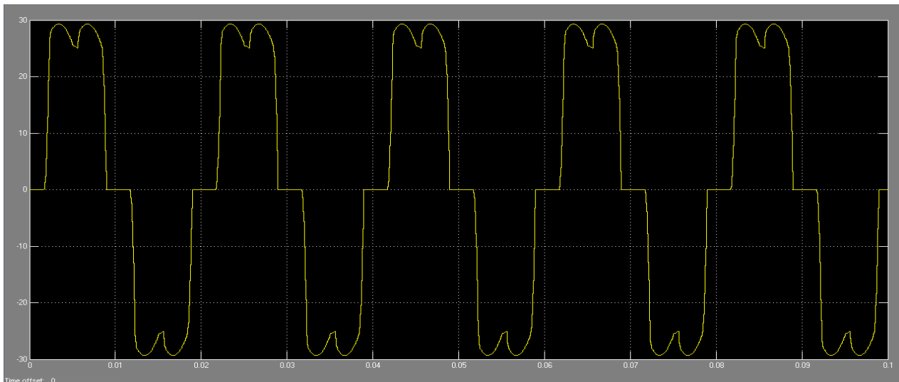
Figure 3.5 Proposed PCC current
