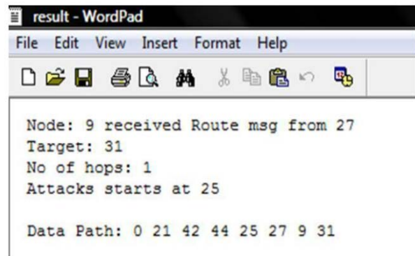
Figure 2:- Path Suggested by AODV protocol in simple scenario without attack
