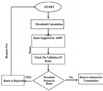
Figure 1: Flow Chart of Proposed Algorithm
