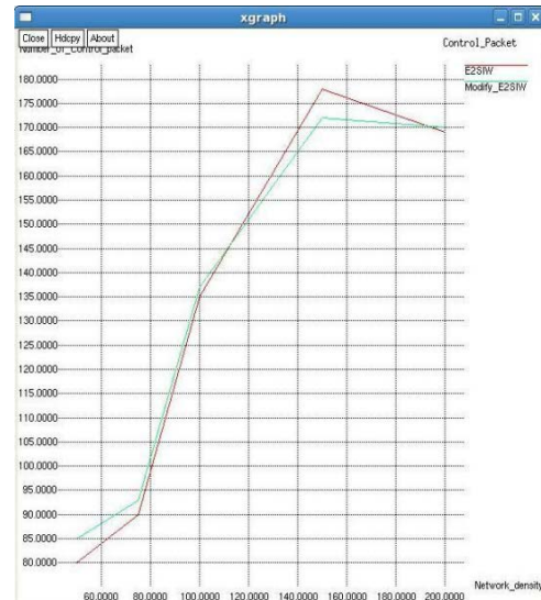
Figure 6: Comparison graph between E2SIW and modify E2SIW for number for control packet
