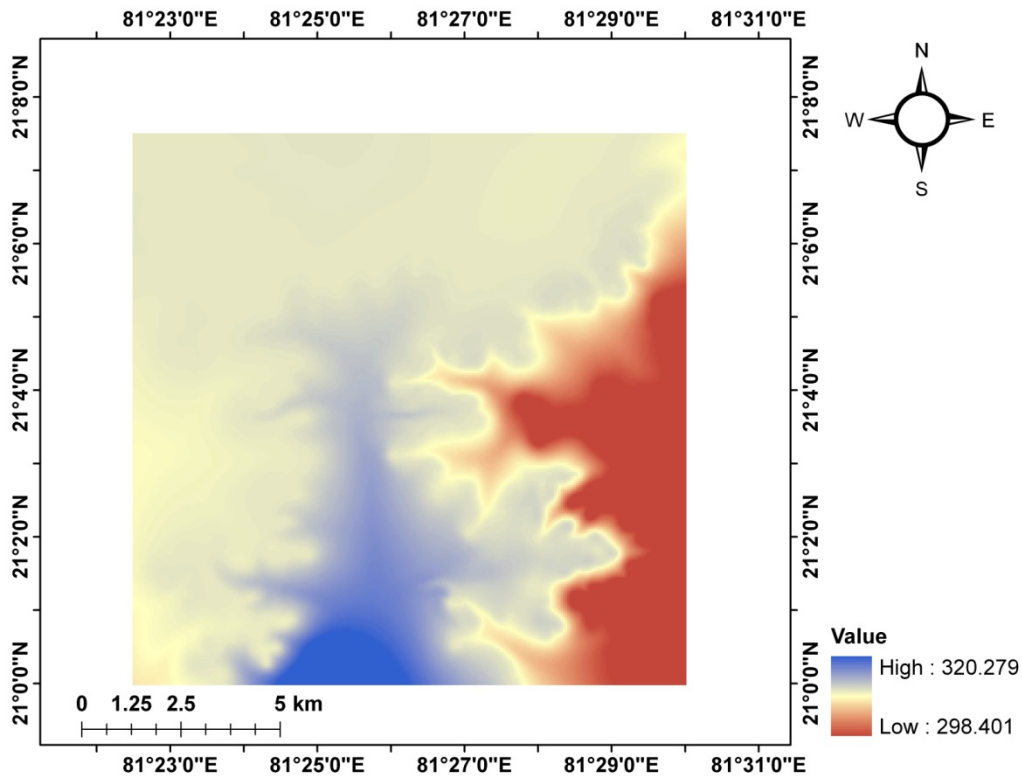
Fig. 4: DEM of Area of Interest using contour lines
