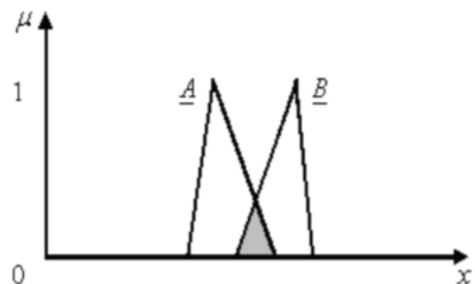
Figure 6: Intersection of Fuzzy sets A and B
