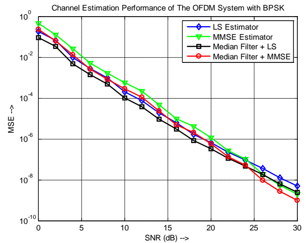
Fig. 4.1 Simulation results of Mean Square Error (MSE) with BPSK Scheme and Median Filter
