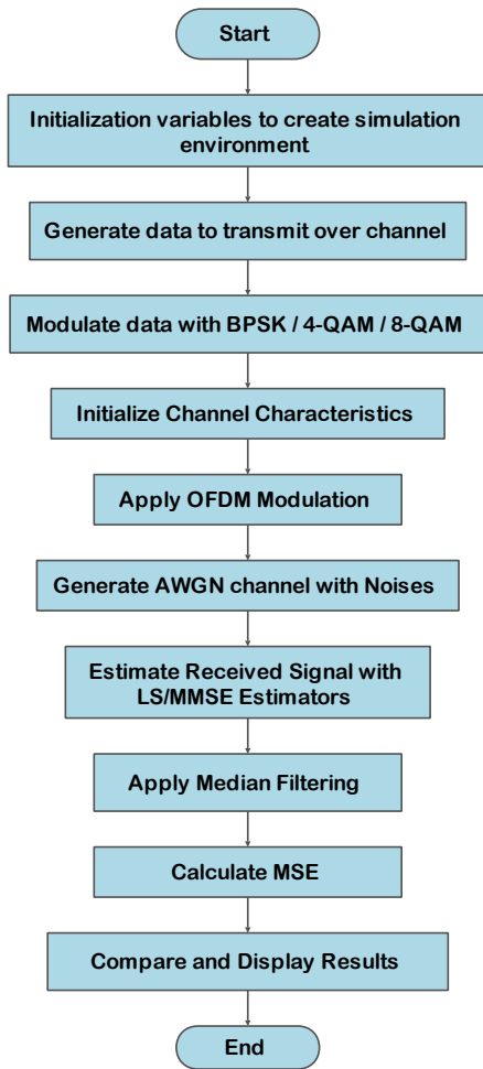
Fig. 3.2 Flow chart of proposed methodology
