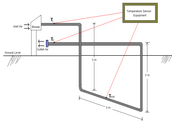
Fig. 4.1: Schematic Representation of Experimental Set up
