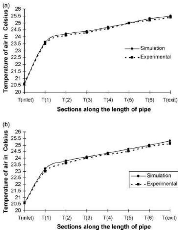
Fig 2.1: Temperature distribution along the length of the pipe for exit velocity 2.0 m/s for (a) steel pipe (b) PVC pipe.
