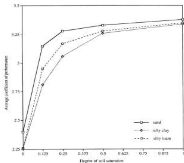
Fig.2.2: Variation of the average COP vs soil degree of saturation.
