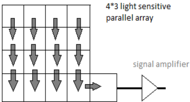
Figure iv. Special cell used for readout [6].
