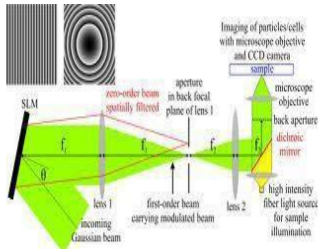
Figure iii. Spatial light modulators [5].
