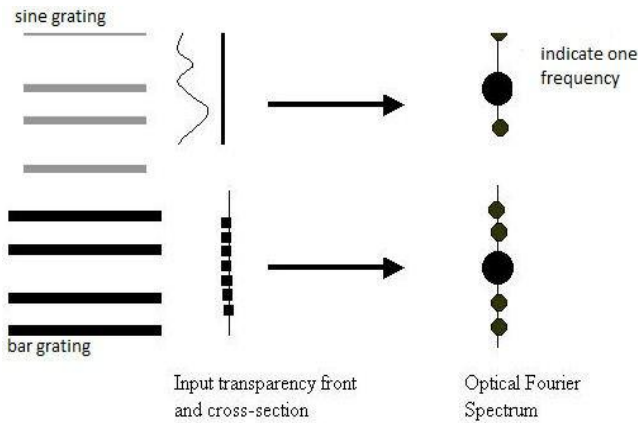
Figure ii. The lens as a Fourier transforms system [4]
