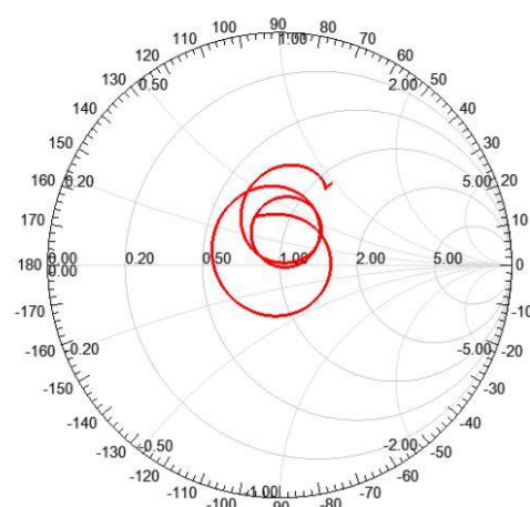
Fig.10. Smith chart
