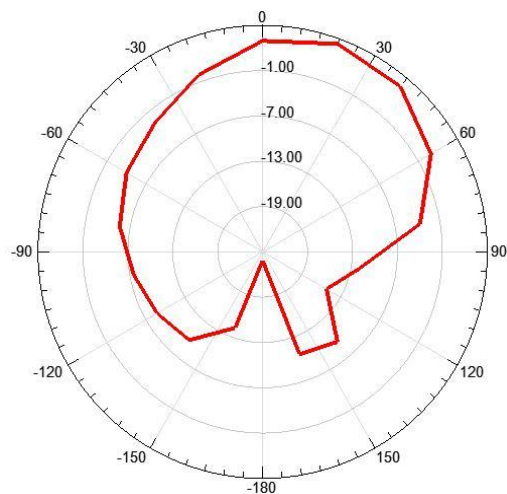
Radiation pattern at phi=0 degrees
