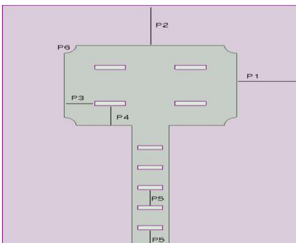
Fig.3.Patch and Feedline
