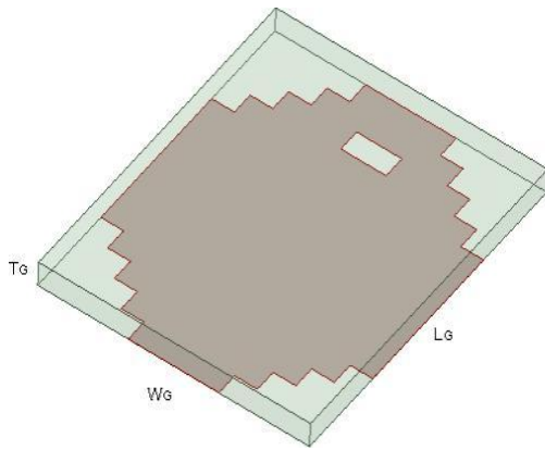
Fig. 2.Substrate Design
