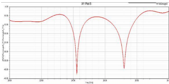
Fig.7.Return Loss plot
