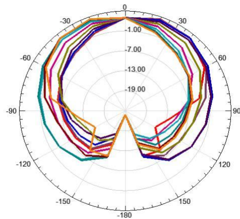
Fig.9.Radiation pattern
