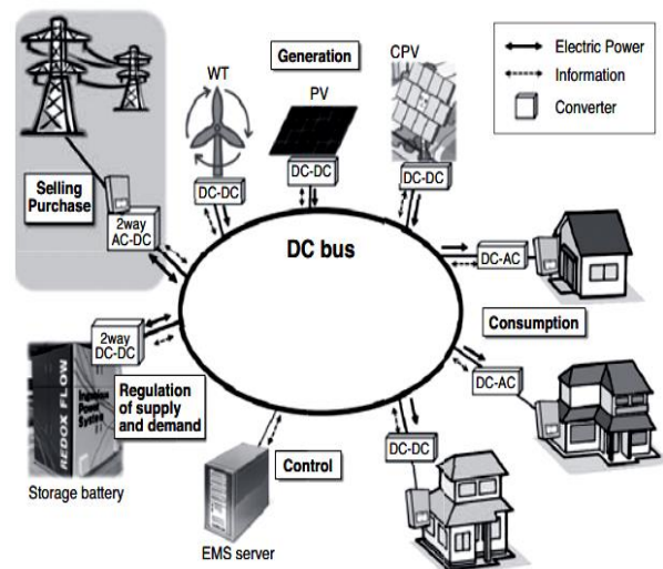
Figure 1: Microgrid Component
