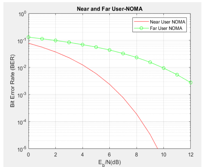
Fig. 12 Average user without proposed algorithm
