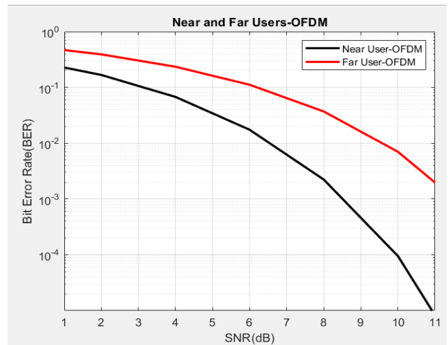
Fig. 11 Near and Far user condition for OFDM
