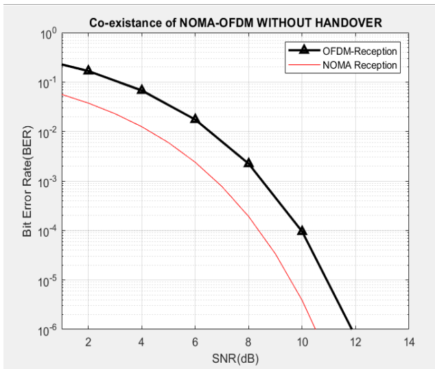
Fig. 13 Co-existence of NOMA-OFDM
