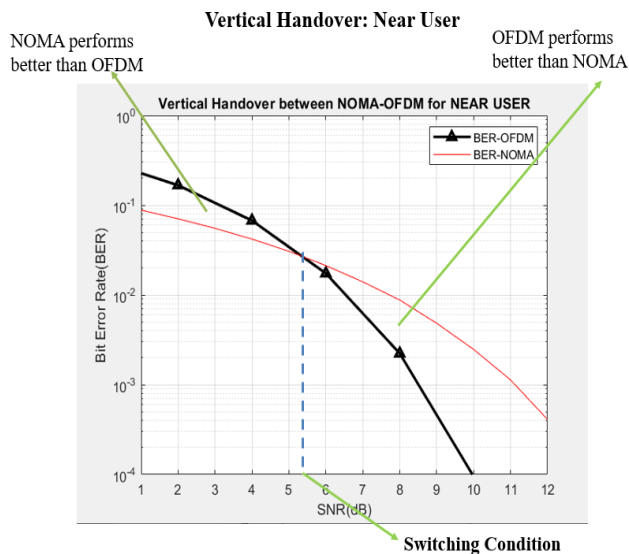
Fig. 14 Vertical handover for near user condition
