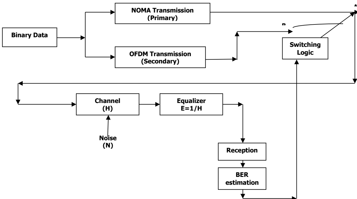
Fig. 3 Proposed Transceiver Design
