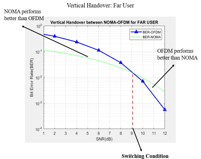
Fig. 15 Vertical handover for far user condition
