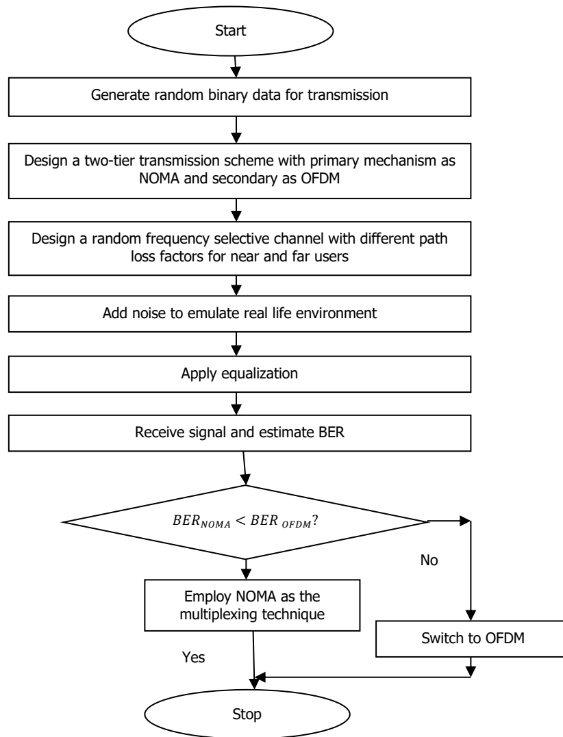
Fig. 4 Flowchart of proposed system
